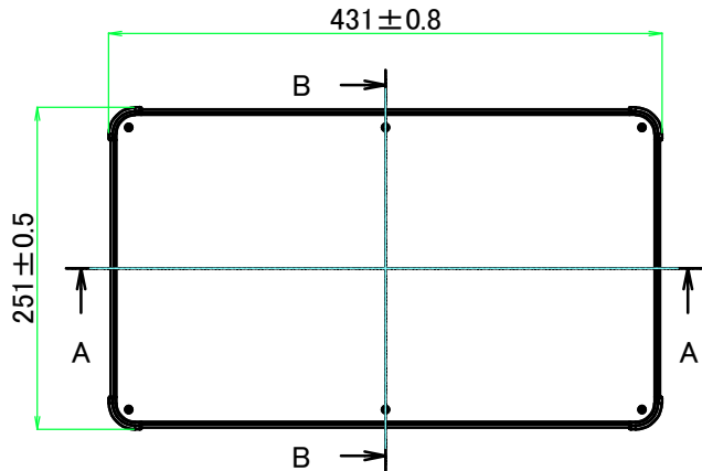
E view
